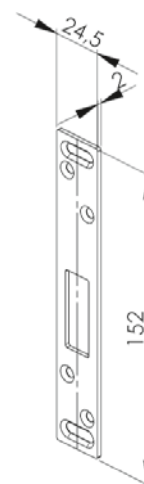
Flat Striking Plate for the hooked bolts
