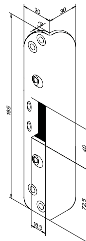
Angled Strikin Plates for the hooked bolts
